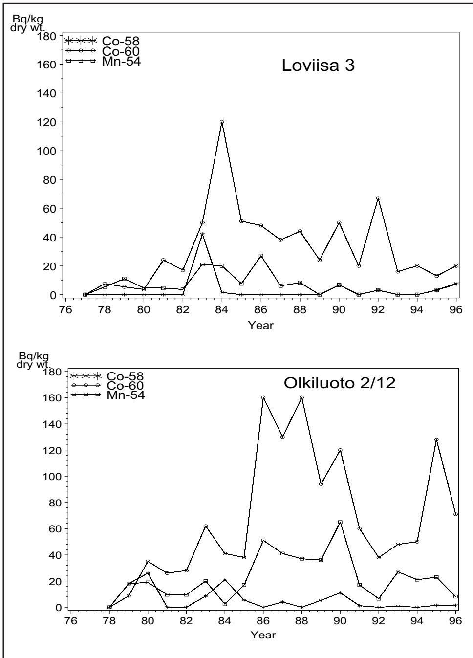
Figure 16. Mean concentrations of ^{54}\text{Mn} , ^{58}\text{Co} and ^{60}\text{Co} in sinking matter at Stations Loviisa 3 and Olkiluoto 2/12 during the open-water period in 1977-1996.
