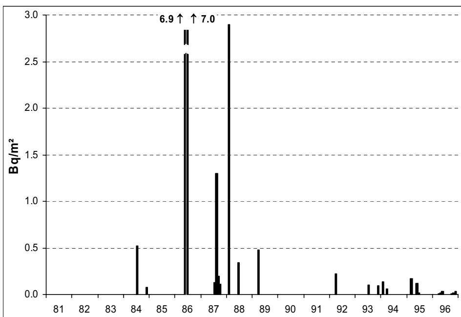
Figure 11. Observations of ^{60}\text{Co} in deposition samples at Station 21, Olkiluoto during 1981-1994.
