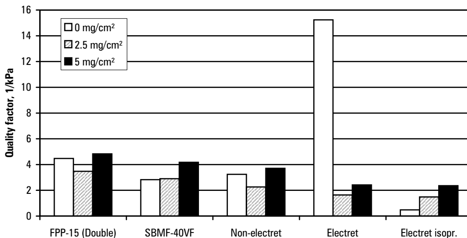
Figure 8. Quality factors for 0.2 \mu\text{m} particles when filters were exposed to 0–5 \text{mg}/\text{cm}^2 of aerosol (the same test runs as in Figure 6).
