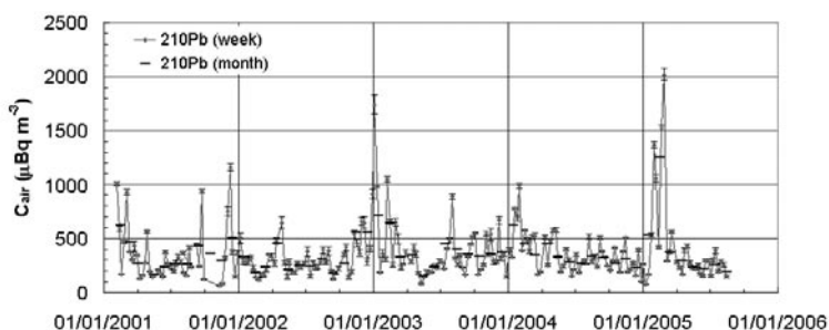
Figure 1. Variation of ^{210}\text{Pb} activity concentration in air, Harku- Tallinn, February 2001 –August 2005: measured weekly values ( \diamond ) and calculated monthly averages ( - ).
