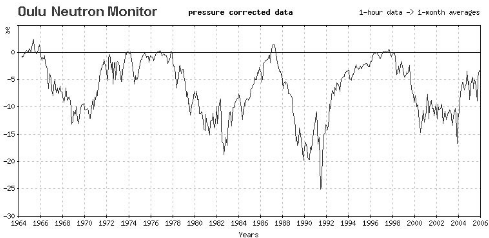
Figure 1. Cosmic ray intensity as measured by the Oulu neutron monitor.
