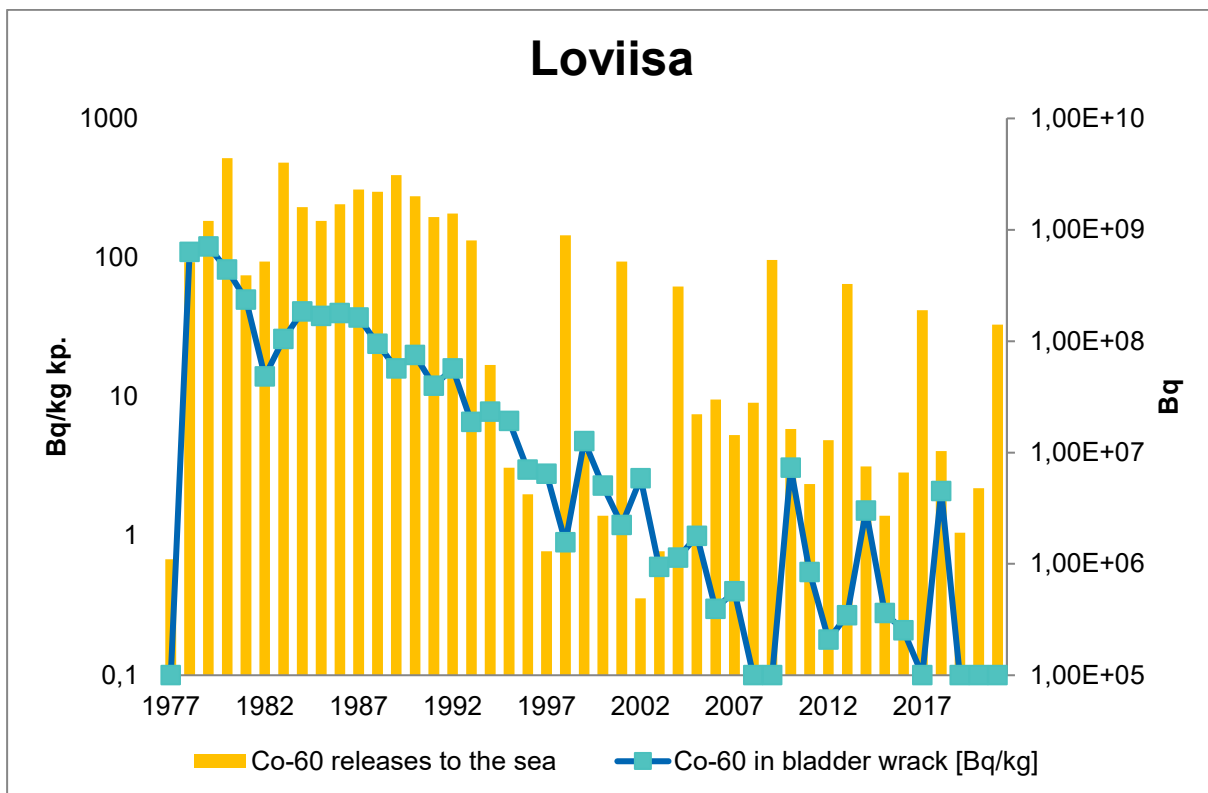
Figure 15. The Co-60 releases into the sea and the average of the Co-60 activity concentration in the bladder wrack samples of the nearest sampling point of the Loviisa power plant in 1977 – 2021.
