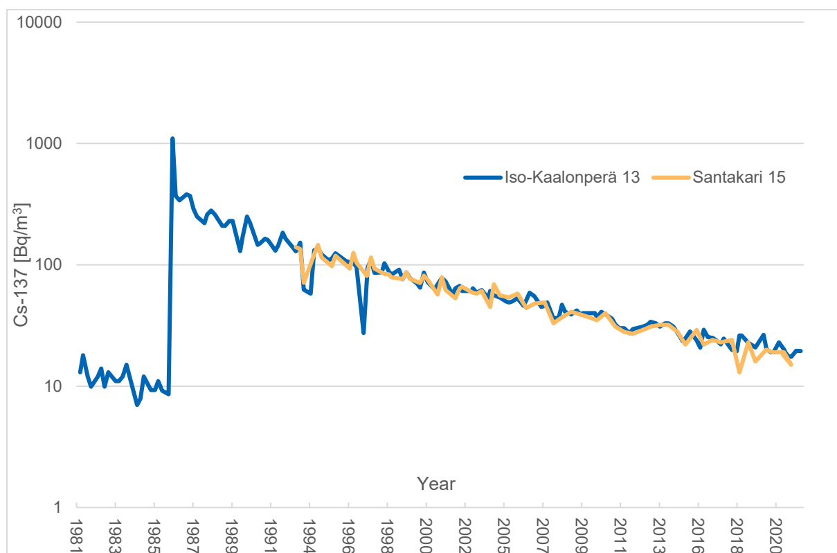
Figure 12. The Cs-137 activity concentration in seawater at the nearest (Iso-Kaalonperä 13, blue) and furthest (Santakari 15, yellow) sampling point of the Olkiluoto power plant in 1981 – 2021 presented on a logarithmic scale.
