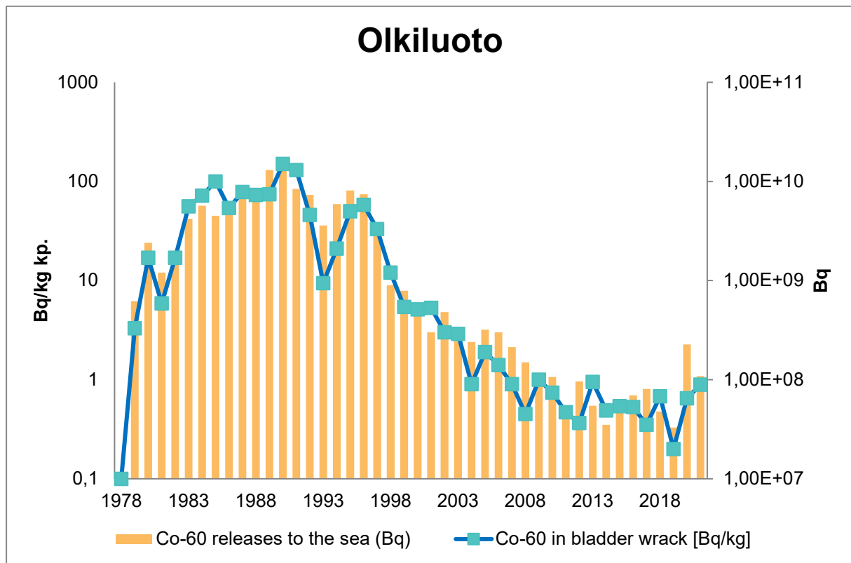
Figure 16. The Co-60 releases into the sea and the average of the Co-60 activity concentration in the bladder wrack samples of the nearest sampling point of the Olkiluoto power plant in 1977 – 2021.
