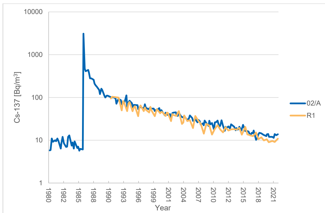
Figure 11. The Cs-137 activity concentration in seawater at the nearest (02/A, blue) and furthest (R1, yellow) sampling point of the Loviisa power plant in 1980 – 2021 presented on a logarithmic scale.
