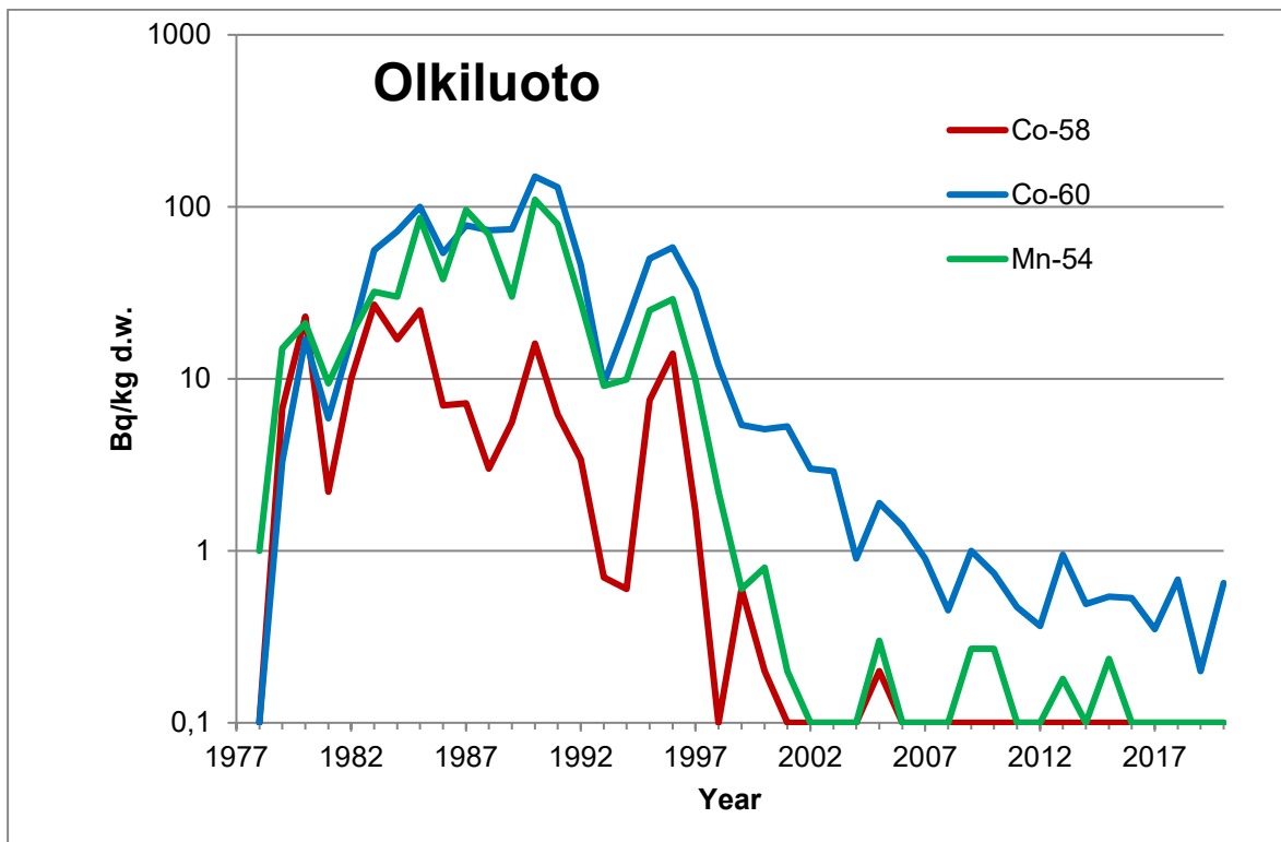
Figure 14. Averages of the activity concentrations of the most significant radionuclides originating from the power plant in bladder wrack (Bq/kg per dry weight) at the nearest sampling point of the Olkiluoto power plant in 1977 – 2021 on a logarithmic scale.
