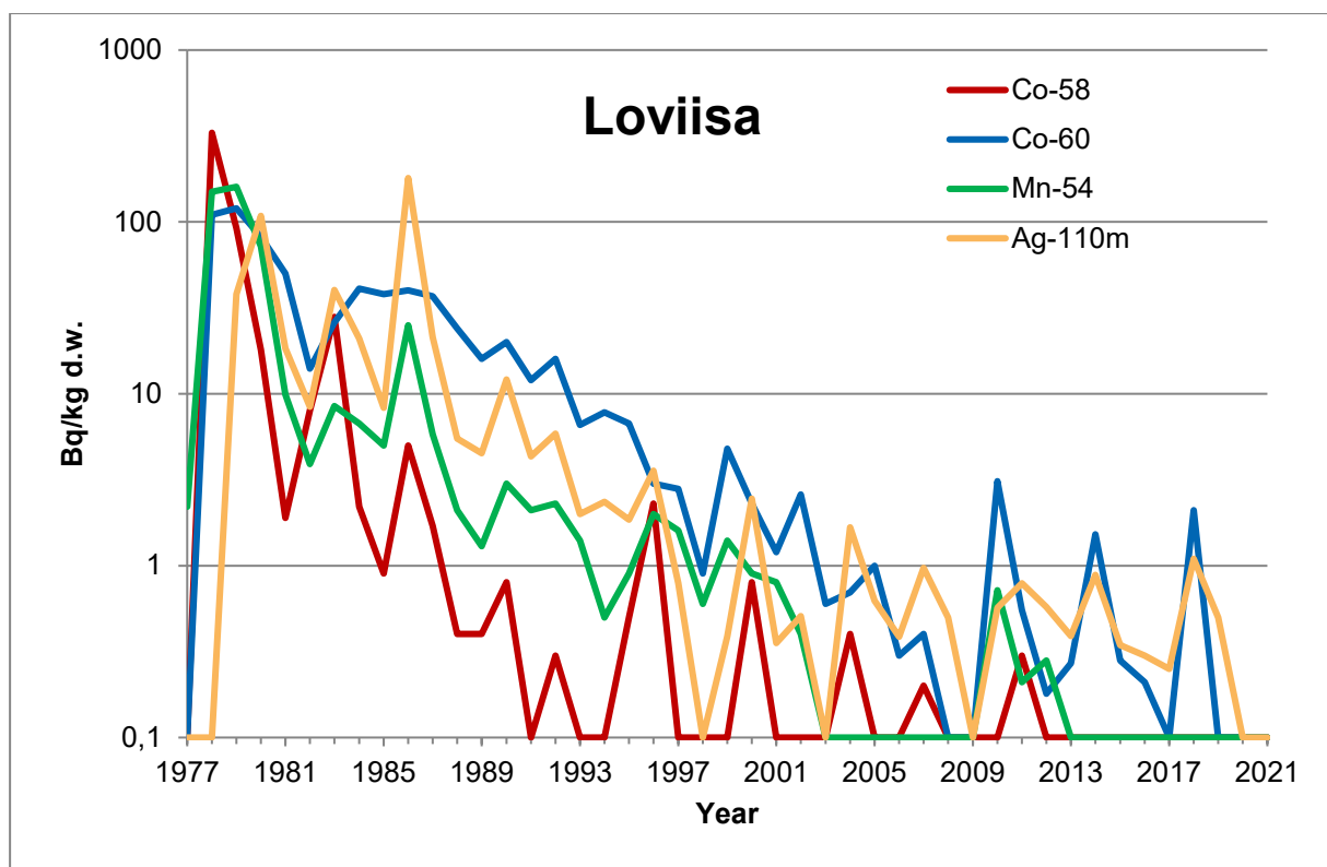
Figure 13. Averages of the activity concentrations of the most significant radionuclides originating from the power plant in bladder wrack (Bq/kg per dry weight) at the nearest sampling point of the Loviisa power plant in 1977 – 2021 on a logarithmic scale.
