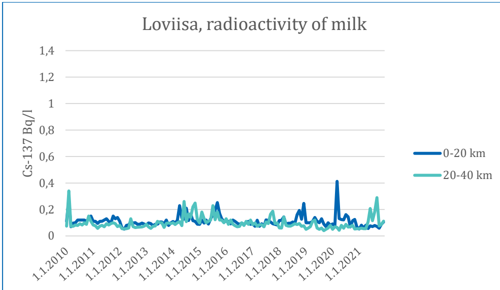
Figure 9. The Cs-137 concentration (Bq/l) of the milk samples supplied by dairies in the surroundings of the Loviisa power plant (distance of the farms from the plant 0 – 20 km or 20 – 40 km) in 2010 – 2021.
